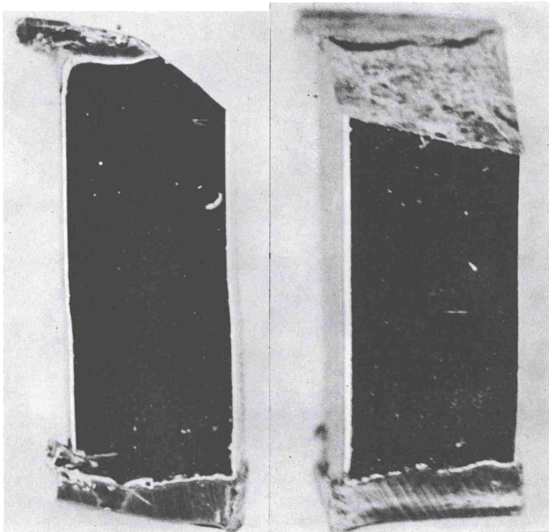
Fig. 10 - Macroscopic Photograph Showing \{11\bar{2}0\} and \{10\bar{1}0\} Lateral Surfaces of Crystal ISR-12 After c-axis Compression Under Hydrostatic Pressure in the Range 261-293 ksi. Mag. 15X
